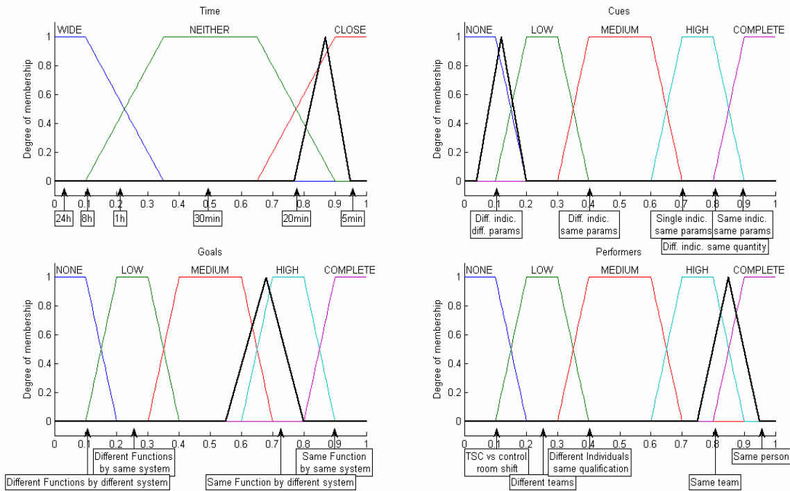
Figure 7. UOD partitioned by trapezoidal FSs. The thick-line triangle represents the FS of the Fact in input to the model
