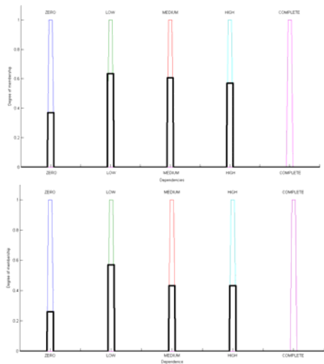
Figure 9. Output FSs of dependence level: input partition by trapezoidal FSs (top) and triangular FSs (bottom).
